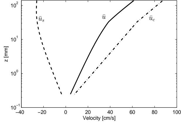
FIGURE 20. Decomposing of the total current velocity profile of test SP400a_C40_sa into a boundary layer streaming and a basic current velocity (solid line: total mean velocity, dashed line: boundary layer streaming, dash-dot line: basic current).
