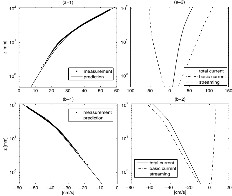
FIGURE 22. Predicted and measured current velocity profile of a C40 current following and opposing the ST400a wave over the sandpaper bottom: (a-1) predicted and measured current velocity profiles for ST400a_C40_sa, (a-2) Decomposition of the predicted current velocity profile for test ST400a_C40_sa, (b-1) predicted and measured current velocity profiles for ST400a_C40r_sa, (b-2) Decomposition of the predicted current velocity profile for test ST400a_C40r_sa.
