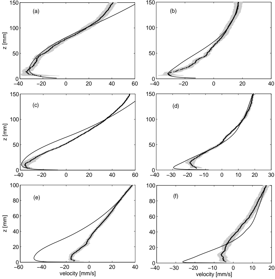
FIGURE 15. Prediction of the boundary layer streaming of the nonlinear waves (black dots: measurements, gray zones: standard deviations given by spatial averaging, solid lines: prediction): (a) ST400a_ce, (b) FL320a_ce, (c) ST400a_sa, (d), FL320a_sa, (e) ST400a_sm, (f) FL320a_sm
