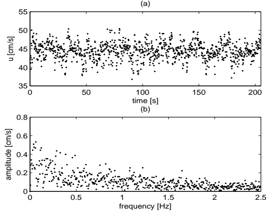
FIGURE 2. Spatial-average velocity of 40Hz test measured at 90mm above the "sandpaper" bottom: (a) time series, (b) frequency spectrum.
