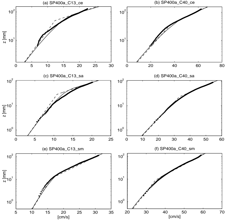
FIGURE 18. Prediction of current velocity profiles in the presence of sinusoidal waves (solid lines: the present model, dashed lines: the improved GM model, dots: measurements): (a) SP400a_C13_ce, (b) SP400a_C40_ce, (c) SP400a_c13_sa, (d) SP400a_c40_sa, (e) SP400a_c13_sm, (f) SP400a_c40_sm.
