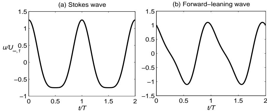
FIGURE 1. Free-stream velocities of nonlinear waves: (a) Stokes wave, (b) Forward-leaning wave.
