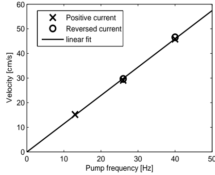
FIGURE 3. Cross-section average current velocities under different pump rotation frequencies (crosses: current in positive direction, open circles: current in negative direction, solid line: a linear fit).
