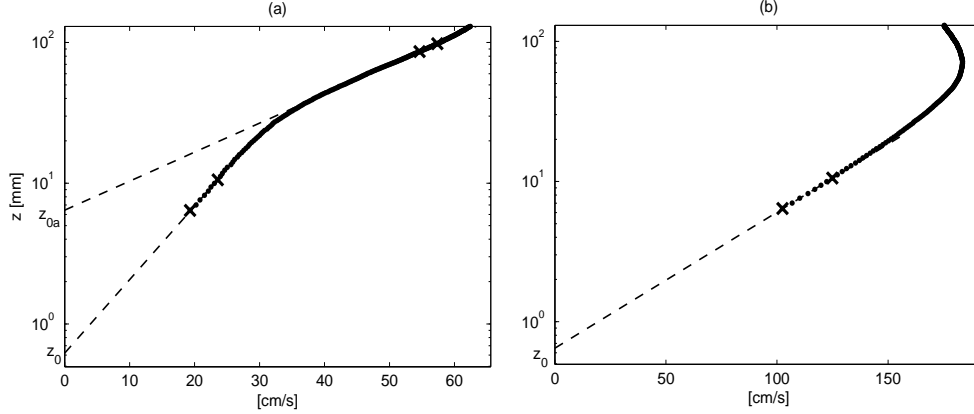
FIGURE 5. Velocity profiles of test SP400a_C40_ce: (a) current velocity profile, (b) first-harmonic amplitude profile (dots: measurements, dashed lines: fitted logarithmic profiles, crosses: limits for selecting data points for log-profile fitting).
