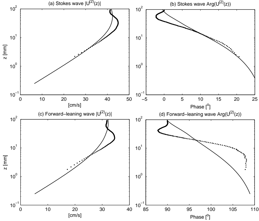
FIGURE 13. Prediction of the second-harmonic velocity of test ST400a_sa (Stokes wave) and FL320a_sa (forward-leaning waves) (solid lines: predictions, dots: measurements): (a) second-harmonic amplitude of test ST400a_sa, (b) second-harmonic phase of test ST400a_sa, (c) second-harmonic amplitude of test FL320a_sa, (d) second-harmonic phase of test FL320a_sa
