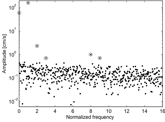
FIGURE 4. Frequency spectrum of spatial-averaged free-stream velocity of test SP400a_C40_sa (frequency is normalized by the wave frequency 0.16Hz).
