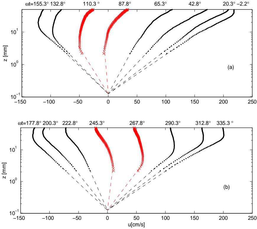
FIGURE 6. Instantaneous Reynolds-averaged velocity profiles of test SP400a_C40_sa and the associated modified log-profile fittings with k_b=3.7\text{mm} (red crosses: measurements with questionable log-profile fittings, dots: measurements with good log-profile fittings, dashed lines: fitted logarithmic profiles ): (a) first half period, (b) second half period.
