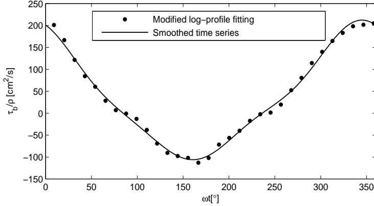
FIGURE 7. The bottom shear stress of test SP400a_C40_sa (full circles: Modified log-profile fitting with bottom roughness k_b=3.7\text{mm} , solid line: smoothed time series for modified log-profile fitting).
