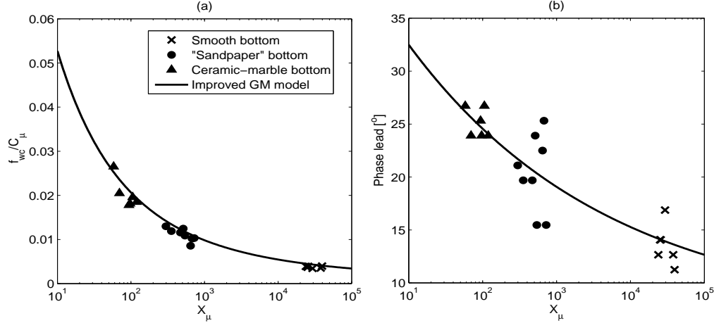
FIGURE 8. Wave friction factors and phase leads of the maximum wave bottom shear stress of combined sinusoidal-wave-current flows (crosses: smooth-bottom tests, circles: sandpaper-bottom tests, triangles: ceramic-marble-bottom tests, solid line: the improved GM model): (a) wave friction factors, (b) phase leads.
