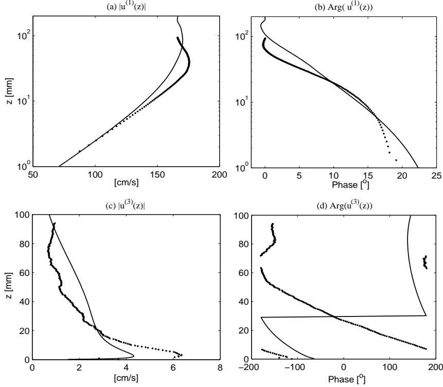
FIGURE 12. Prediction of the first- and third-harmonic velocities of sinusoidal wave test SP400a_sa (solid lines: predictions, dots: measurements): (a) first-harmonic amplitude, (b) first-harmonic phase, (c) third-harmonic amplitude, (d) third-harmonic phase
