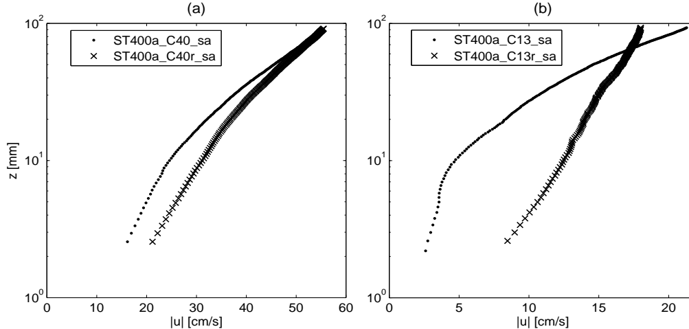
FIGURE 9. Magnitudes of measured current velocity profiles of the ST400a wave plus currents over the “sandpaper” bottom (dots: positive currents (in the wave direction), crosses: negative currents (against the wave direction): (a) strong (C40) currents, (b) weak (C13) currents
