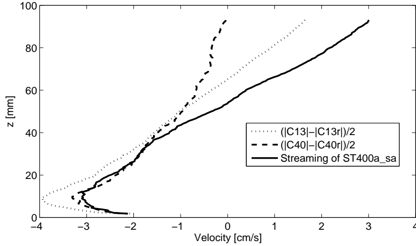
FIGURE 10. Estimate of the embedded mean velocity of test ST400a_sa (dotted line: based on C13 currents, dashed line: based on C40 current, solid line: measured mean velocity of test ST400a_sa).
