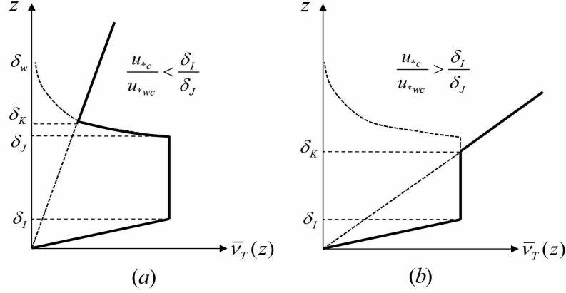
FIGURE 11. Vertical structure of the time-averaged turbulent eddy viscosity for oscillatory turbulent boundary layer flows: (a) weak current, (b) strong current.
