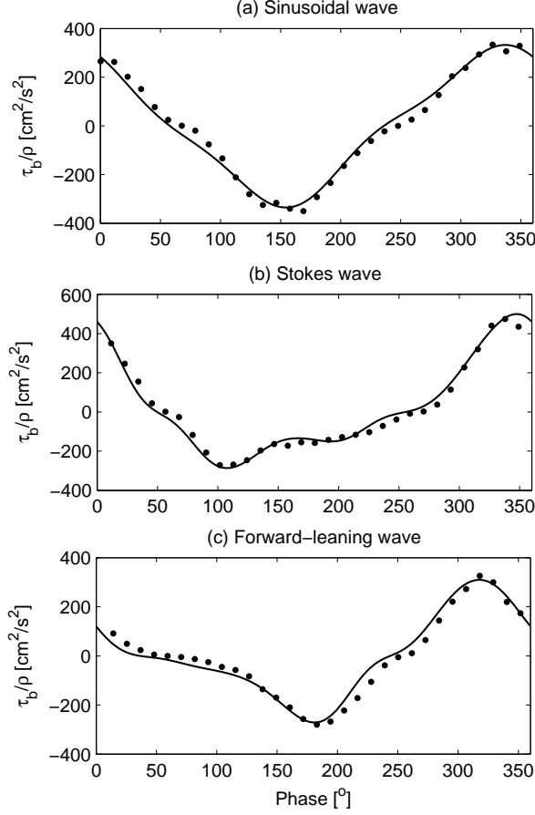
FIGURE 14. Prediction of wave bottom shear stress (solid lines: predictions, dots: measurements from modified log-profile fitting analysis with k_b=3.7\text{mm} ): (a) test SP400a_sa (sinusoidal wave), (b) test ST400a_sa (Stokes wave), (c) test FL320_sa (forward-leaning wave).
