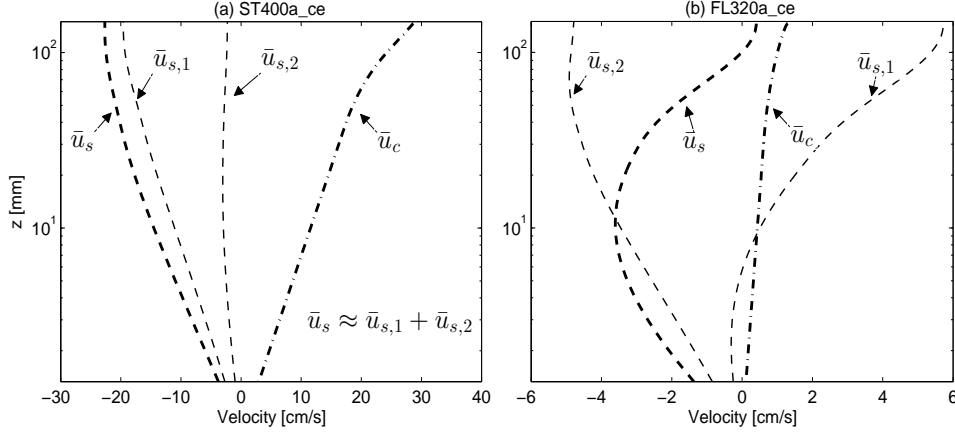
FIGURE 16. Decomposing of the mean velocity profile embedded in nonlinear waves (thick dashed lines: turbulence asymmetry streaming, thin dashed lines: main components of turbulence asymmetry streaming, thick dash-dot lines: basic (return) current): (a) Stokes wave (ST400a_ce), (b) forward-leaning wave (FL320a_ce)
