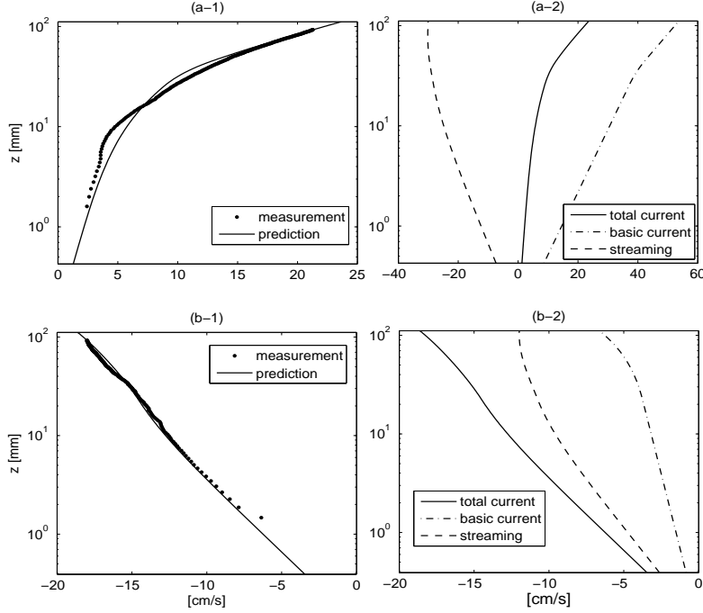
FIGURE 21. Predicted and measured current velocity profile of a C13 current following and opposing the ST400a wave over the sandpaper bottom: (a-1) predicted and measured current velocity profiles for ST400a_C13_sa, (a-2) Decomposition of the predicted current velocity profile for test ST400a_C13_sa, (b-1) predicted and measured current velocity profiles for ST400a_C13r_sa, (b-2) Decomposition of the predicted current velocity profile for test ST400a_C13r_sa.
