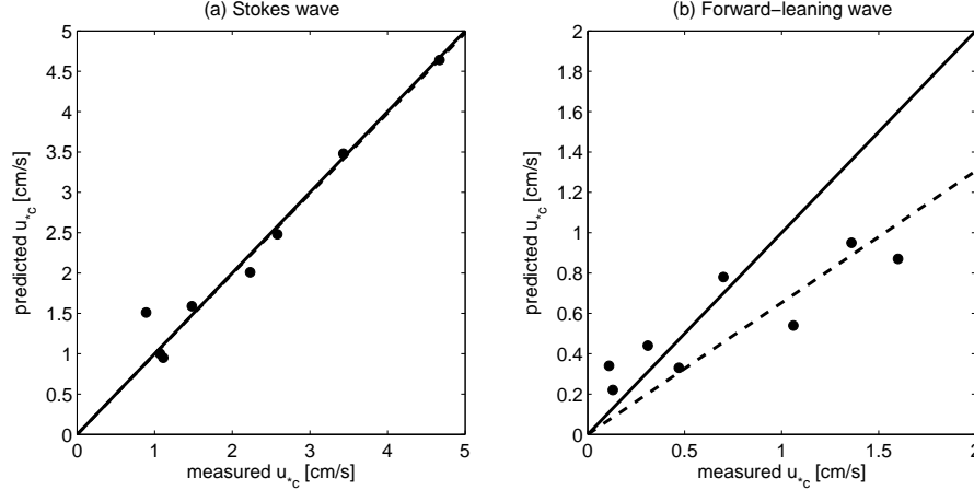
FIGURE 17. Comparison of the predicted and measured current shear velocity for nonlinear waves (solid line: perfect agreement, dashed lines: least-square fit to the data): (a) Stokes waves, (b) forward-leaning waves.
